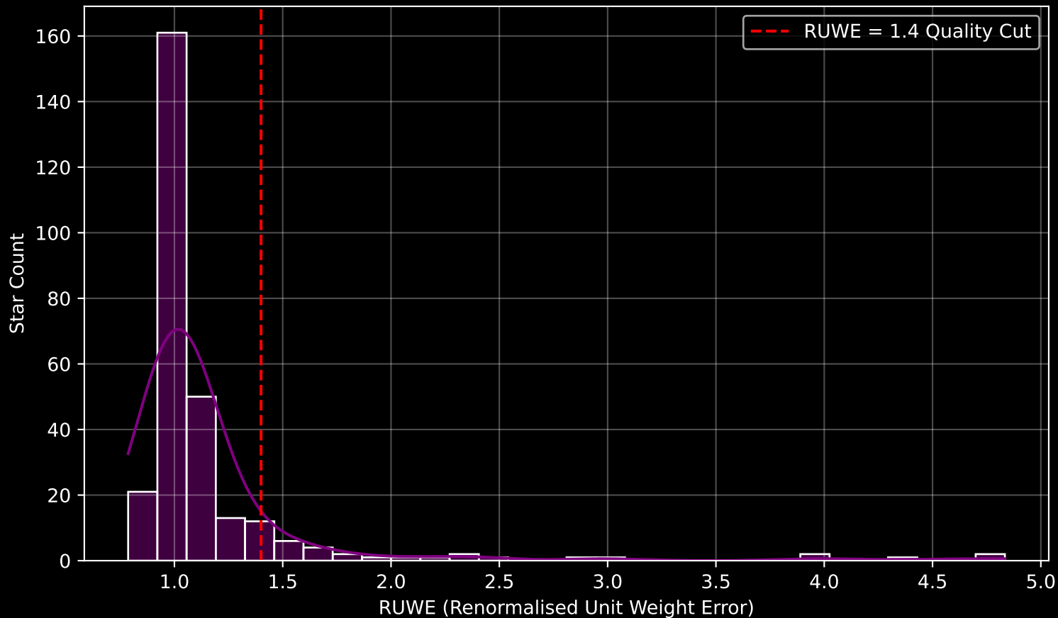
GALAH DR4 Field [1239] RUWE Distribution (n= 282)
