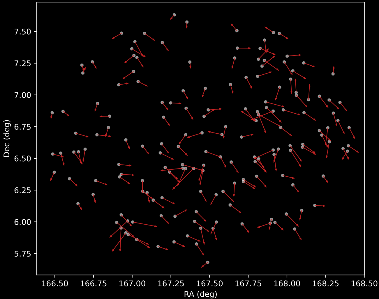
GALAH DR4 Cluster 6 Proper Motion Vectors (n=165)
