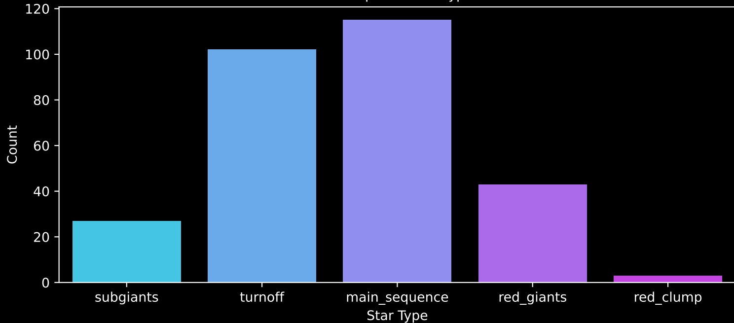
GALAH DR4 Field: [1239] Count plot of Star Type
