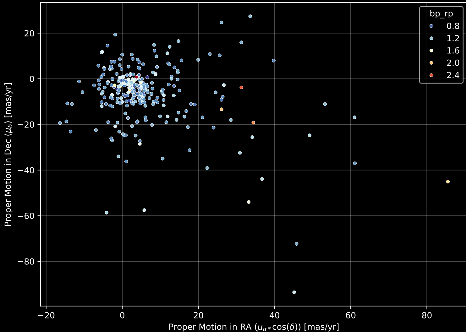
GALAH DR4 Field: [1239] Proper Motion Diagram (n= 290)
