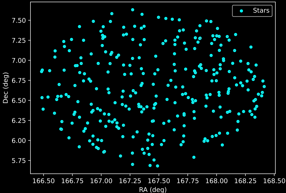
GALAH DR4 Field: [1239] Proper Motion Vectors for Gaia Star Field (n= 290)
